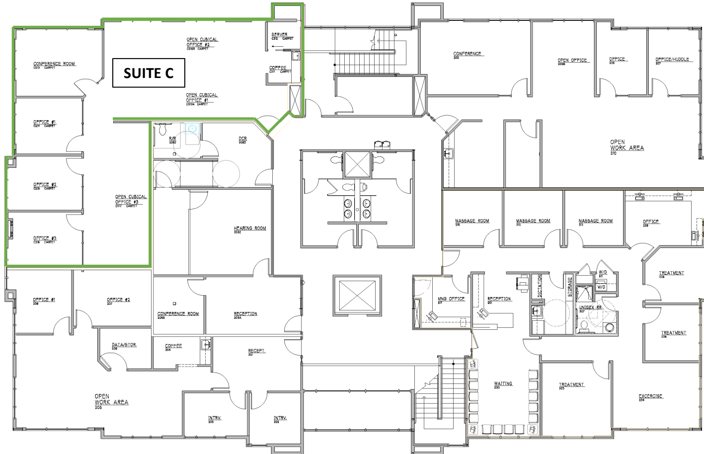
SECOND FLOOR PLAN 1/4" = 1'-0" 52728X_FPS
